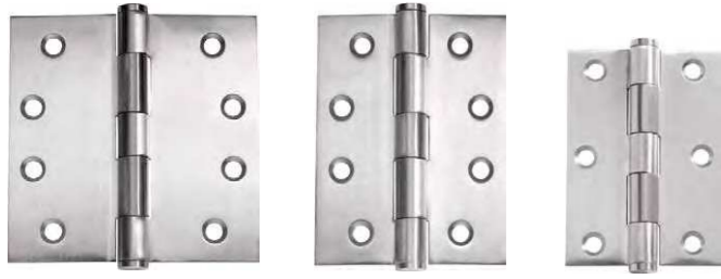
2874 SS W100xH100xT2.5mm 2873 SS W75xH100xT2.5mm 2872 SS W60xH85xT2mm
